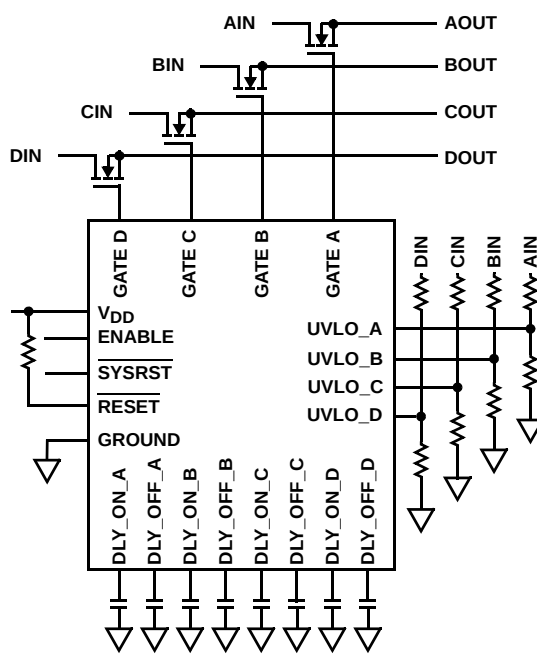
FIGURE 1. TYPICAL ISL6123 APPLICATION
