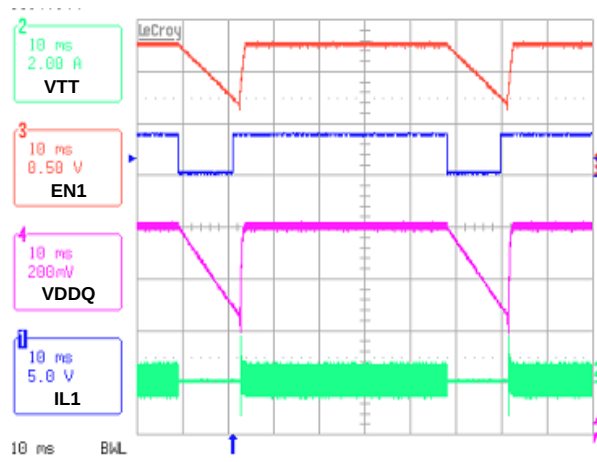
FIGURE 30. VTT FOLLOWS VDDQ, ENABLE 2 IS HIGH
