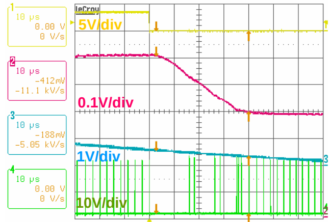
FIGURE 26. V BOOT TO V VID , V IN = 19V, I O = 2A, V VID = 0.7625V, Ch1: CLK_EN#, Ch2: V O , Ch3: PMON, Ch4: PHASE
