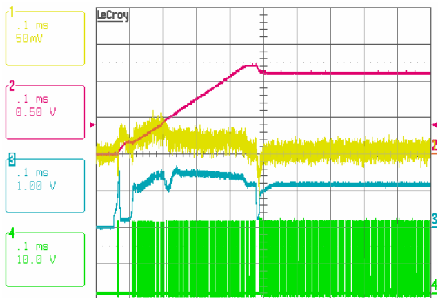
FIGURE 29. SOFT START INRUSH CURRENT, V IN = 19V, I O = 2A, V VID = 1.1V, Ch1: DROOP-V O (2.1mV = 1A), Ch2: V O , Ch3: V comp , Ch4: PHASE
