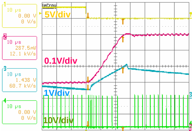
FIGURE 25. V BOOT TO V VID , V IN = 19V, I O = 2A, V VID = 1.5V, Ch1: CLK_EN#, Ch2: V O , Ch3: PMON, Ch4: PHASE
