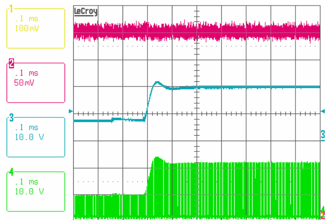
FIGURE 30. V IN TRANSIENT TEST, V IN = 8→19V, I O = 2A, V VID = 1.1V, Ch2: V O , Ch3: V IN , Ch4: PHASE
