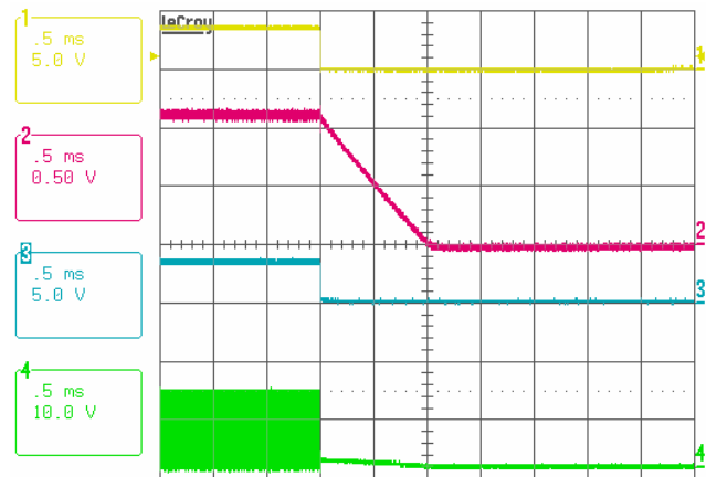
FIGURE 28. SHUT DOWN, V IN = 12.6V, I O = 2A, V VID = 1.1V, Ch1: VR_ON, Ch2: V O , Ch3: PGOOD, Ch4: PHASE
