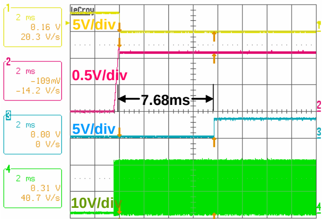
FIGURE 27. CLK_EN AND PGOOD ASSERTION DELAY, V IN = 19V, I O = 2A, V VID = 1.1V, Ch1: CLK_EN#, Ch2: V O , Ch3: PGOOD, Ch4: PHASE
