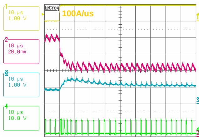
FIGURE 33. LOAD STEP UP RESPONSE IN CCM, V_{IN} = 8V , I_o = 2A \rightarrow 20A at 100A/μs, VID = 1.1V, Ch1: I_o , Ch2: Vo, Ch3: Vcomp, Ch4: PHASE
