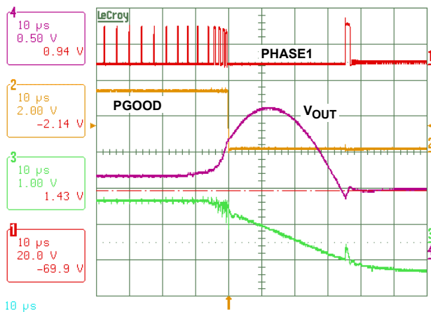
FIGURE 25. 1.7V OVERVOLTAGE PROTECTION SHOWS OUTPUT VOLTAGE PULLED LOW TO 0.9V AND PWM THREE-STATE
