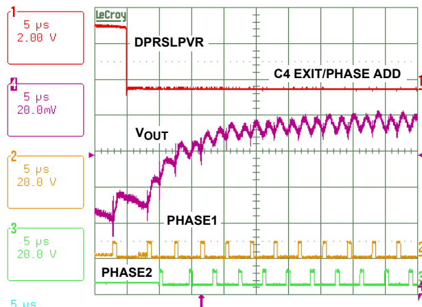
FIGURE 21. VID3 CHANGE OF 010X000 FROM 1V TO 1.1V WITH DPRSLPVR = 0, DPRSTP# = 1, PSI# = 1
