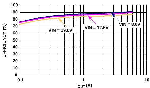
FIGURE 8. EFFICIENCY OF 1-PHASE DE MODE, \text{PSI}_I = \text{LOW} , DCM MODE, \text{VID} = 0.9\text{V} , \text{OFFSET} = 33\text{mV}
