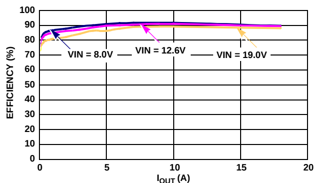
FIGURE 6. ACTIVE MODE EFFICIENCY, 1 PHASE, DE, \text{PSI}_L = \text{LOW} , V_{ID} = 1.15\text{V}
