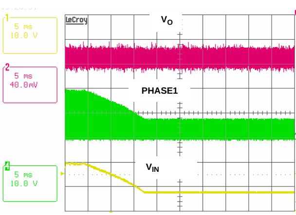
FIGURE 15. 19V TO &gt;8V INPUT LINE TRANSIENT RESPONSE AT ILOAD = 5A AND VID = 1.15V
