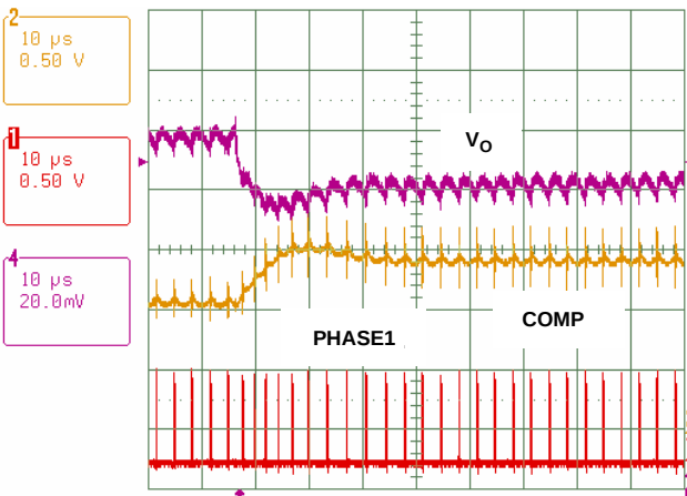
FIGURE 18. LOAD APPLICATION RESPONSE AT 1-PHASE DE MODE, I_{LOAD} = 4A \rightarrow 19A , PSI_L = 0 , AND V_{ID} = 1V
