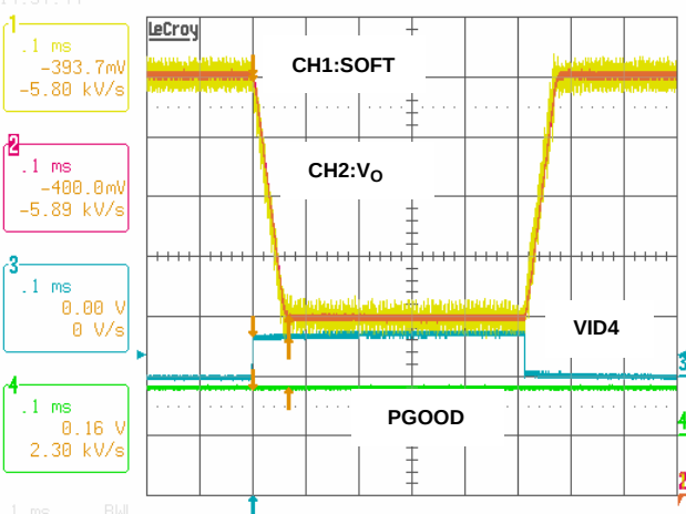
FIGURE 20. VID TRANSITION RESPONSE AT 2-PHASE CCM MODE, V_{IN} = 12.6V AND V_{ID} = 1.55V \rightarrow 1.15V
