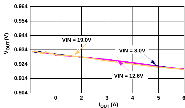
FIGURE 9. 1-PHASE DE MODE LOAD LINE, \text{PSI}_I = \text{LOW} , \text{VID} = 0.9\text{V} , \text{OFFSET} = 33\text{mV}
