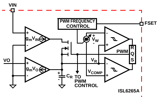
FIGURE 5. MODULATOR CIRCUITRY
