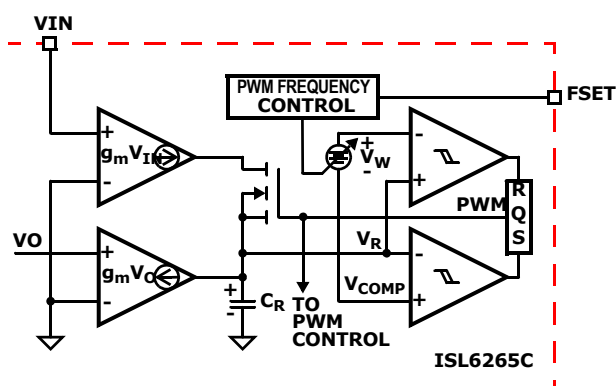
FIGURE 5. MODULATOR CIRCUITRY
