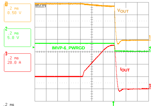
FIGURE 23. OVERCURRENT PROTECTION
