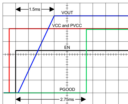
FIGURE 4. SOFT-START SEQUENCE
