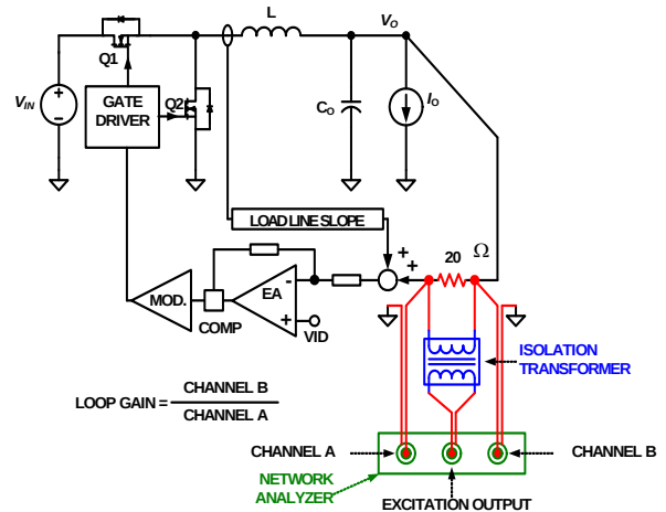
FIGURE 31. LOOP GAIN T2(s) MEASUREMENT SET-UP
