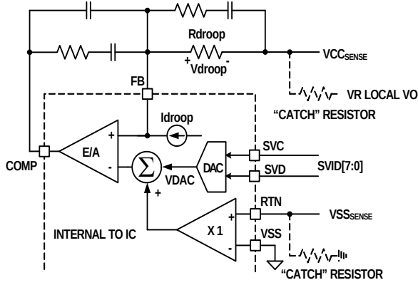
FIGURE 14. DIFFERENTIAL SENSING AND LOAD LINE IMPLEMENTATION
