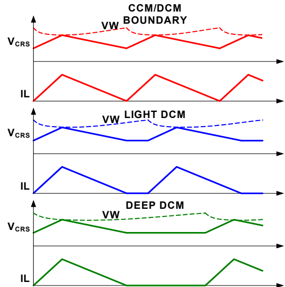
FIGURE 11. PERIOD STRETCHING
