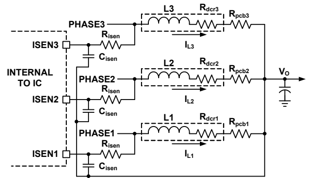
FIGURE 15. CURRENT BALANCING CIRCUIT
