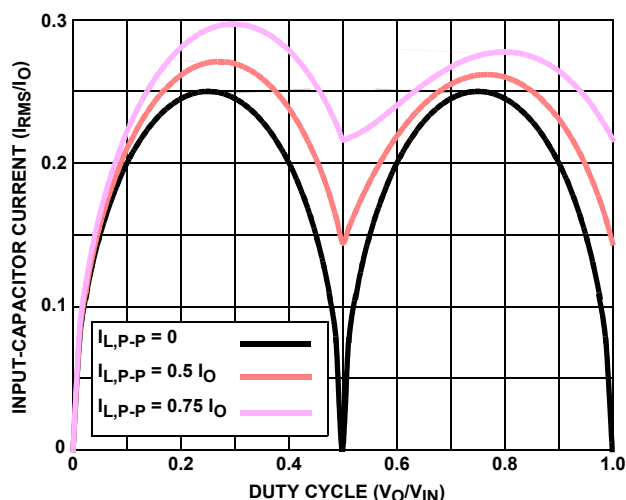
FIGURE 22. NORMALIZED INPUT-CAPACITOR RMS CURRENT vs DUTY CYCLE FOR 2-PHASE CONVERTER
