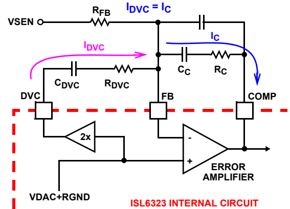
FIGURE 11. DYNAMIC VID COMPENSATION NETWORK
