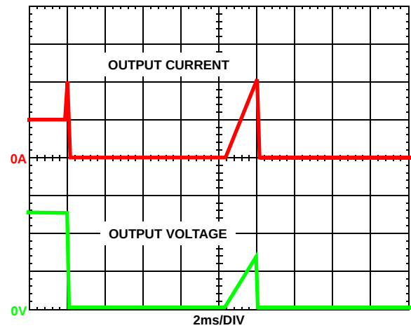
FIGURE 10. OVERCURRENT BEHAVIOR IN HICCUP MODE. F_{SW} = 500kHz
