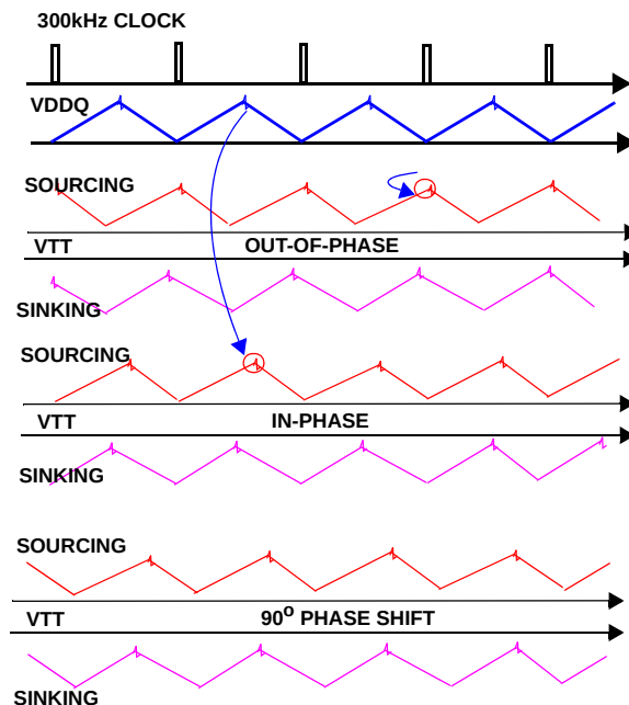
FIGURE 8. CHANNEL INTERFERENCE VIN = 5V
