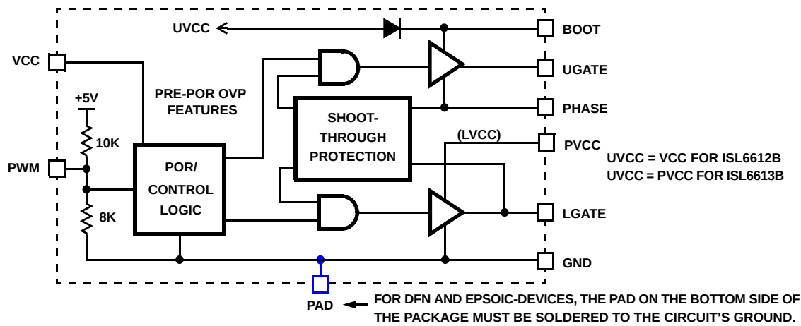
ISL6612B AND ISL6613B
