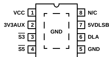
ISL6506 (8 LD EPDIP) TOP VIEW
