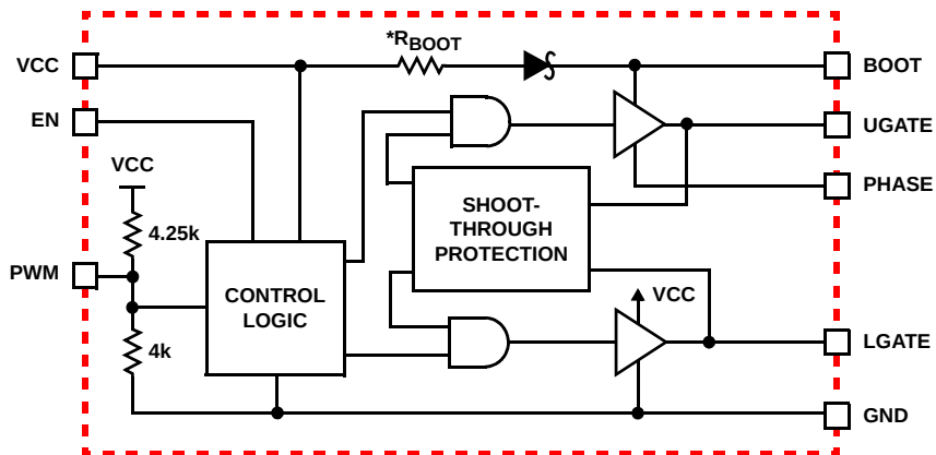
ISL6620, ISL6620A
