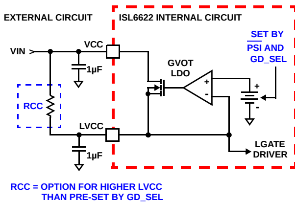
FIGURE 2. GATE VOLTAGE OPTIMIZATION (GVOT) DETAIL
