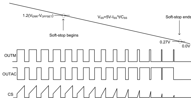
FIGURE 8. SOFT-STOP FUNCTION ( I_{\text{DELAY}} POSITIVE)
