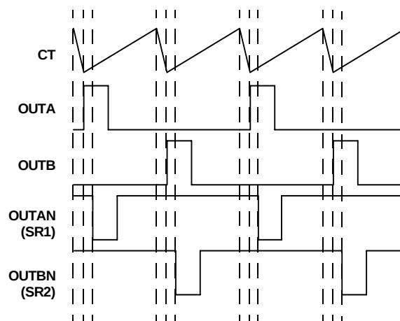
FIGURE 13. WAVEFORM TIMING WITH SR OUTPUTS DELAYED, 2.575\text{V} < \text{VADJ} < 5.00\text{V}
