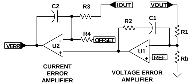
FIGURE 16. AVERAGE CURRENT MODE CONTROL
