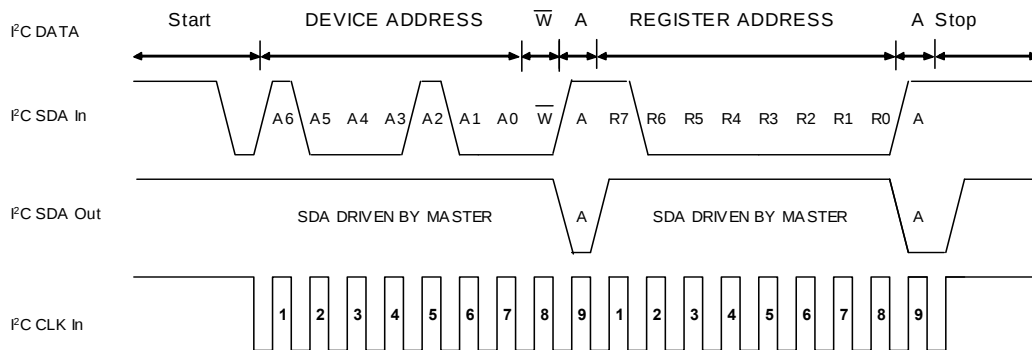
FIGURE 14. I 2 C sync_lic TIMING DIAGRAM SAMPLE
