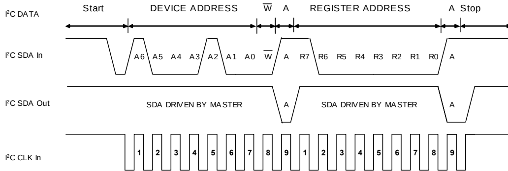
FIGURE 14. I²C sync_lic TIMING DIAGRAM SAMPLE
