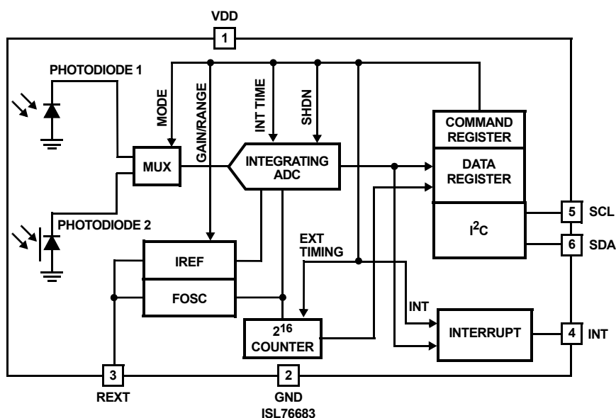
FIGURE 1. BLOCK DIAGRAM
