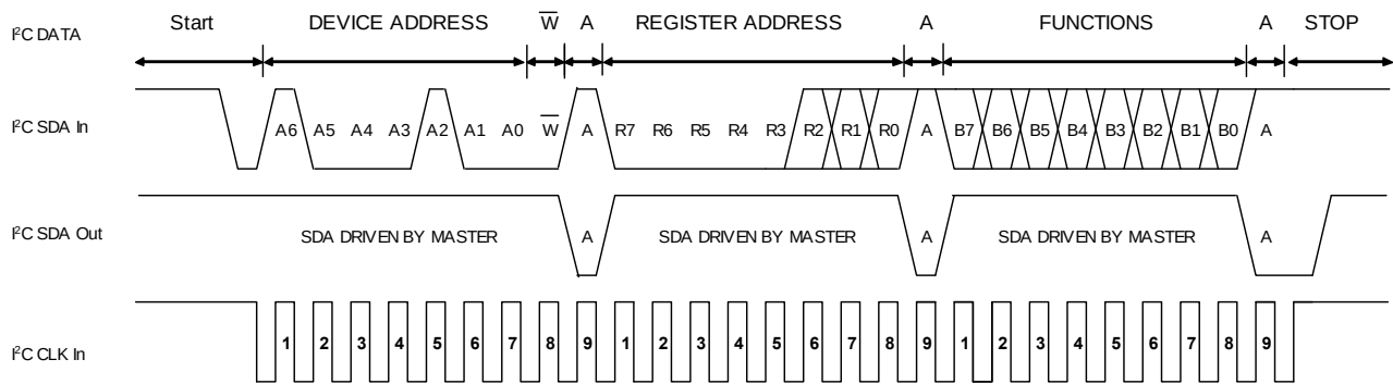
FIGURE 13. I²C WRITE TIMING DIAGRAM SAMPLE
