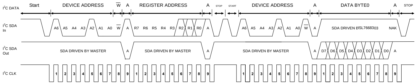
FIGURE 12. I²C READ TIMING DIAGRAM SAMPLE
