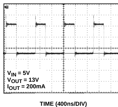
FIGURE 18. LX WAVEFORM - CONTINUOUS MODE
