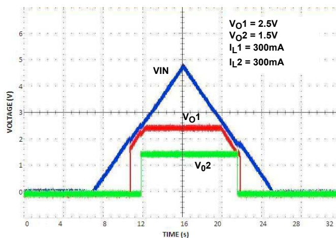
FIGURE 11. POWER-UP/POWER-DOWN
