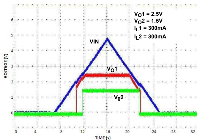
FIGURE 10. POWER-UP/POWER-DOWN
