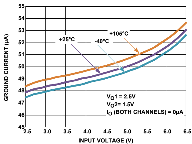
FIGURE 7. GROUND CURRENT vs INPUT VOLTAGE
