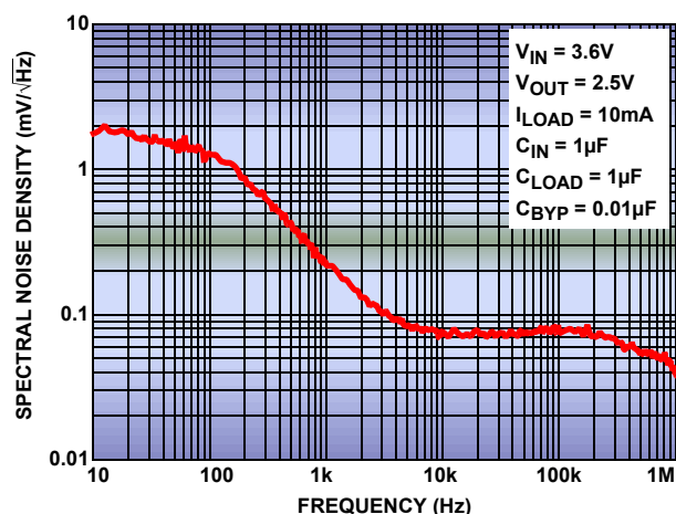
FIGURE 15. SPECTRAL NOISE DENSITY vs FREQUENCY (2.5V OUTPUT, 10mA LOAD)
