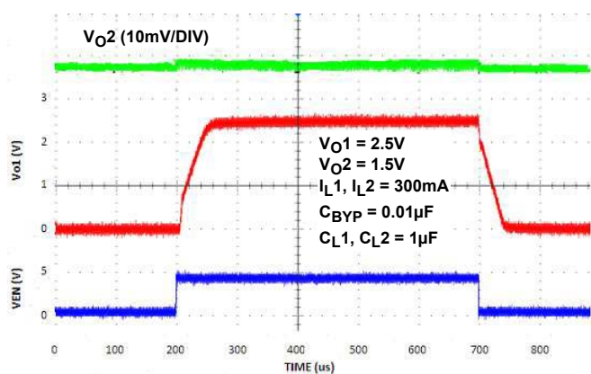
FIGURE 12. TURN-ON/TURN-OFF RESPONSE
