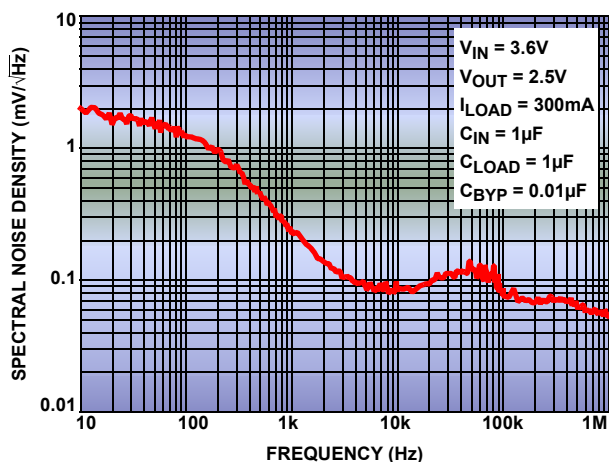
FIGURE 16. SPECTRAL NOISE DENSITY vs FREQUENCY (2.5V OUTPUT, 300mA LOAD)
