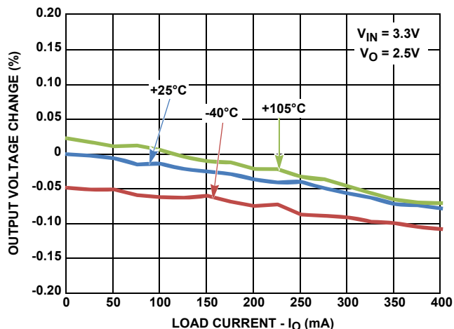
FIGURE 3. LOAD REGULATION
