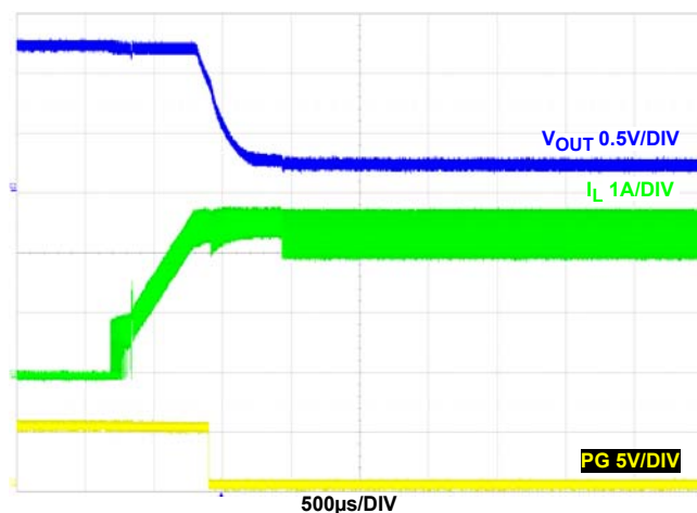
FIGURE 48. OVERCURRENT PROTECTION F_{SW} = 2\text{MHz} , V_{IN} = 5\text{V} , MODE = PWM, T_A = +25^\circ\text{C}
