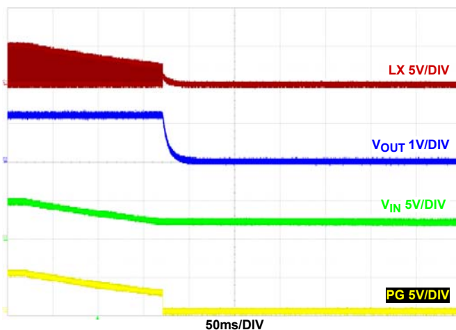
FIGURE 40. SHUTDOWN V_{IN} AT NO LOAD F_{SW} = 2\text{MHz} , V_{IN} = 5\text{V} , MODE = PWM, T_A = +25^\circ\text{C}
