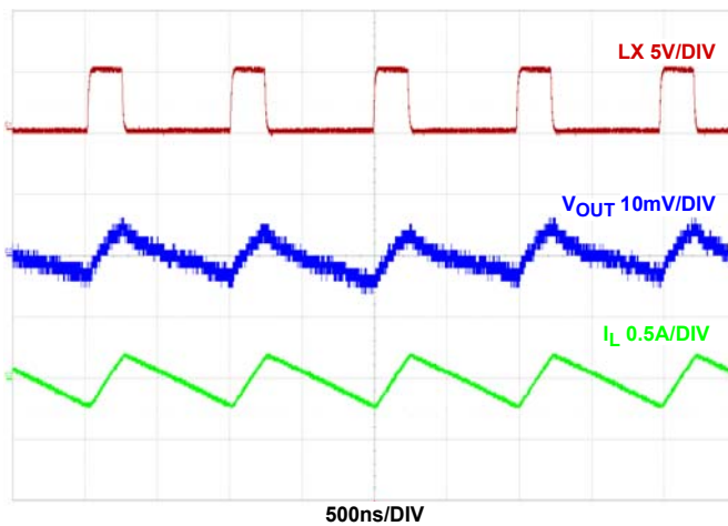
FIGURE 44. STEADY STATE AT NO LOAD F_{SW} = 2\text{MHz} , V_{IN} = 5\text{V} , MODE = PWM, T_A = +25^\circ\text{C}
