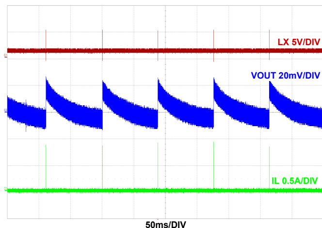
FIGURE 40. STEADY STATE AT NO LOAD F_{SW} = 2\text{MHz} , V_{IN} = 5\text{V} , MODE = PFM, T_A = +25^\circ\text{C}
