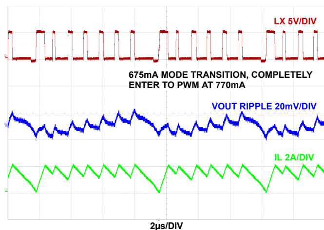
FIGURE 46. PFM TO PWM TRANSITION F_{SW} = 2\text{MHz} , V_{IN} = 5\text{V} , \text{MODE} = \text{PFM} , T_A = +25^\circ\text{C}
