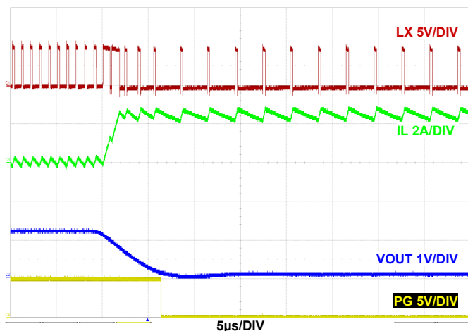
FIGURE 44. OUTPUT SHORT-CIRCUIT F_{SW} = 2\text{MHz} , V_{IN} = 5\text{V} , MODE = PFM, T_A = +25^\circ\text{C}
