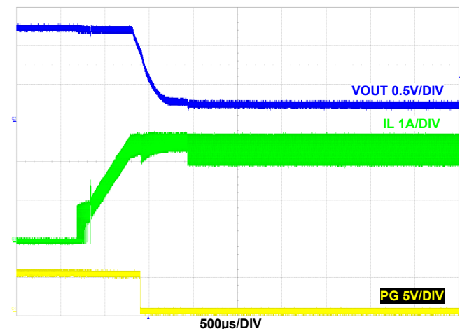
FIGURE 45. OVERCURRENT PROTECTION F_{SW} = 2\text{MHz} , V_{IN} = 5\text{V} , MODE = PWM, T_A = +25^\circ\text{C}
