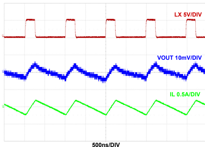
FIGURE 41. STEADY STATE AT NO LOAD F_{SW} = 2\text{MHz} , V_{IN} = 5\text{V} , MODE = PWM, T_A = +25^\circ\text{C}
