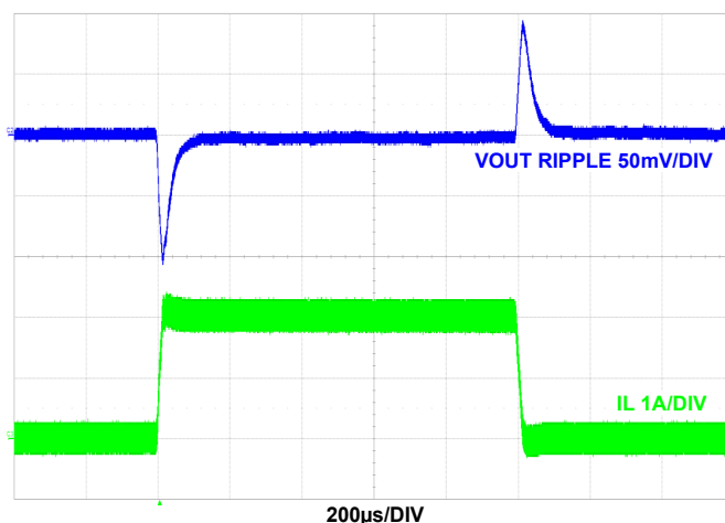
FIGURE 43. LOAD TRANSIENT F_{SW} = 2\text{MHz} , V_{IN} = 5\text{V} , MODE = PWM, T_A = +25^\circ\text{C}
