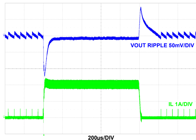
FIGURE 42. LOAD TRANSIENT F_{SW} = 2\text{MHz} , V_{IN} = 5\text{V} , MODE = PFM, T_A = +25^\circ\text{C}
