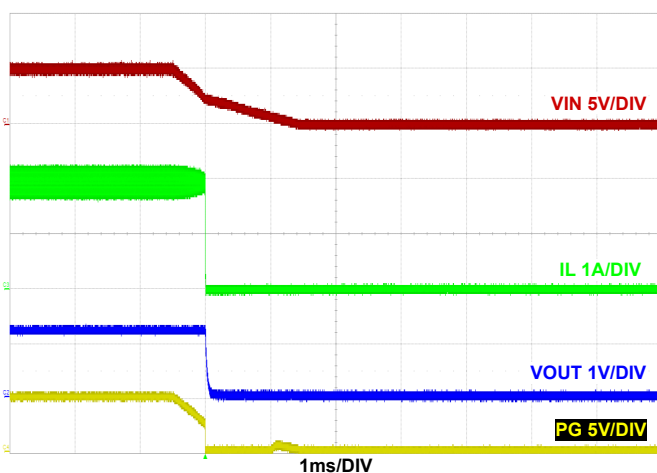
FIGURE 33. SHUTDOWN V_{IN} AT 2A LOAD F_{SW} = 2\text{MHz} , V_{IN} = 5\text{V} , MODE = PWM, T_A = +25^\circ\text{C}
