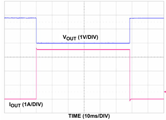
FIGURE 22. CURRENT LIMIT RESPONSE (ISL80102)
