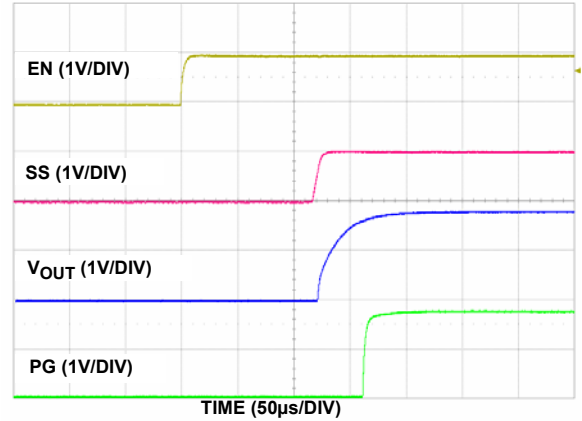
FIGURE 16. ENABLE START-UP
