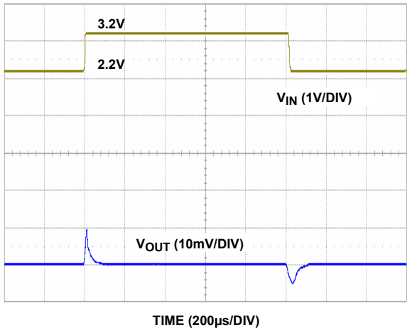
FIGURE 35. LINE TRANSIENT
