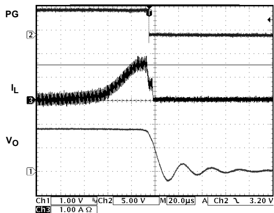
FIGURE 28. OVERCURRENT SHUTDOWN
