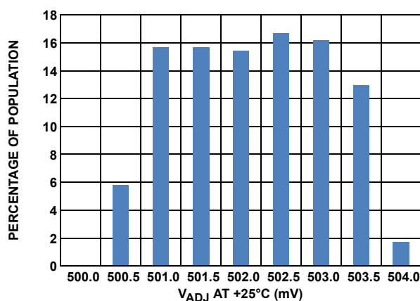
FIGURE 7. V_{ADJ} DISTRIBUTION
