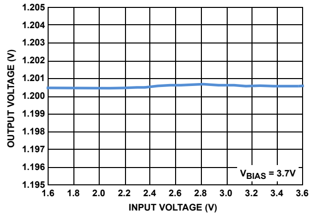
FIGURE 11. V_{\text{IN}} LINE REGULATION
