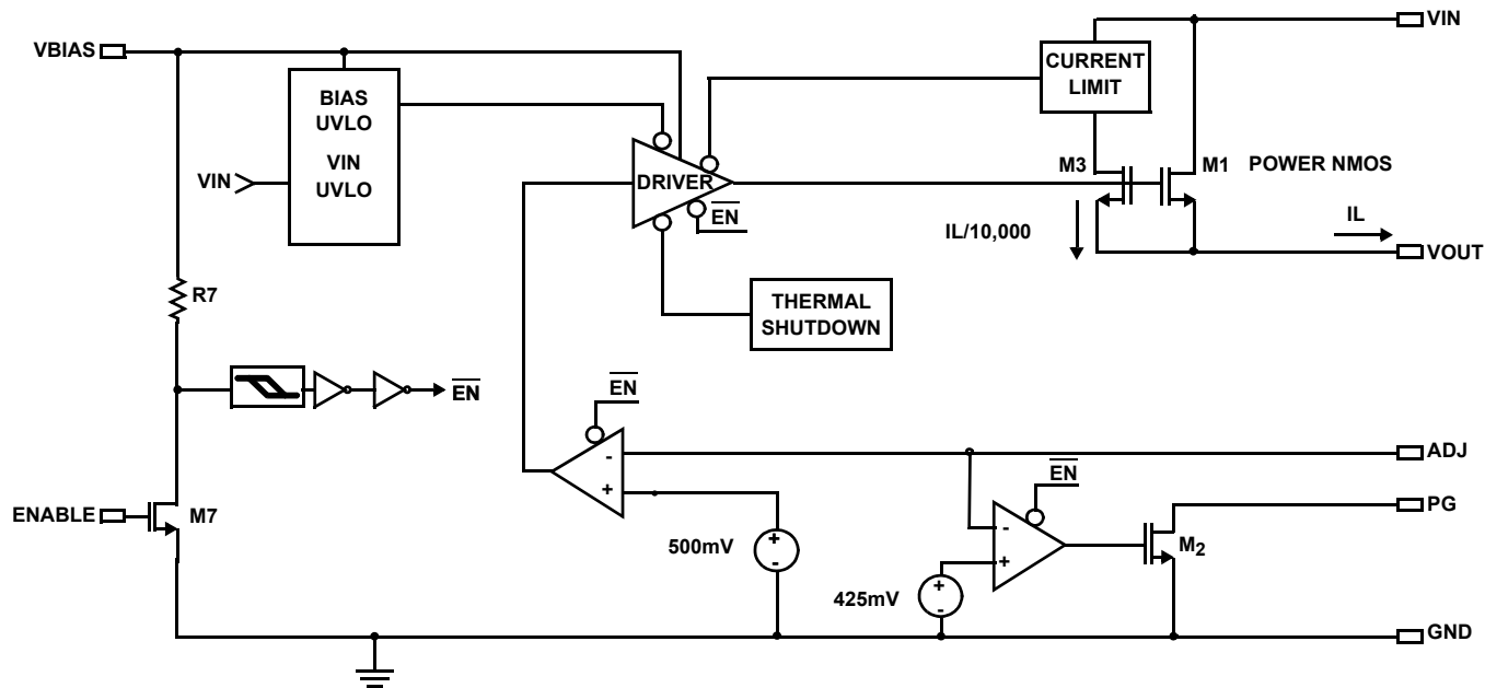
FIGURE 5. BLOCK DIAGRAM
