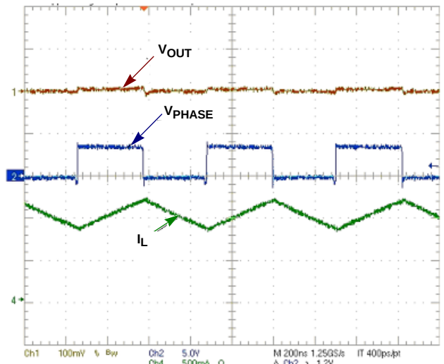
FIGURE 8. STEADY-STATE ( V_{IN} = 3.6V ; V_O = 1.6V ; I_O = 1A )
