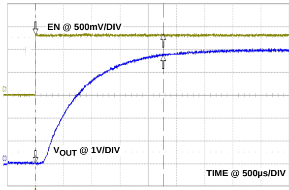
FIGURE 8. START-UP WAVEFORM
