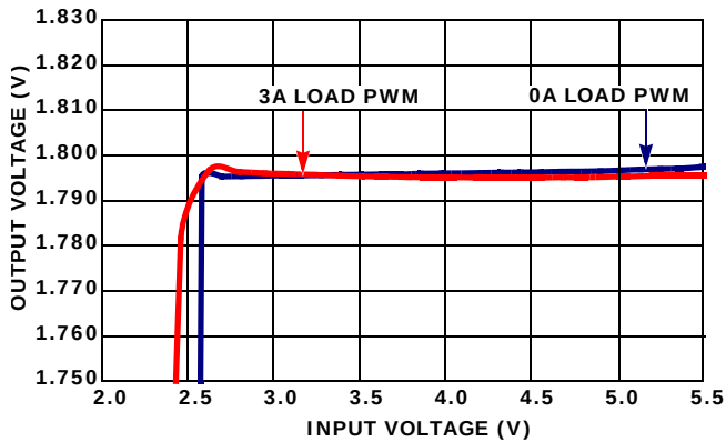
FIGURE 15. OUTPUT VOLTAGE REGULATION vs VIN (PWM V_{\text{OUT}} = 1.8\text{V} )
