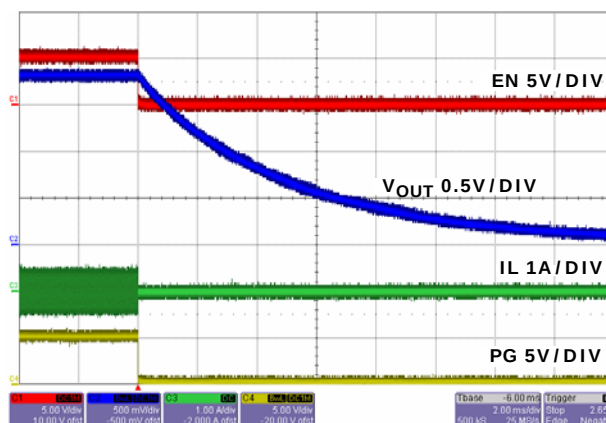
FIGURE 28. SOFT-DISCHARGE SHUTDOWN
