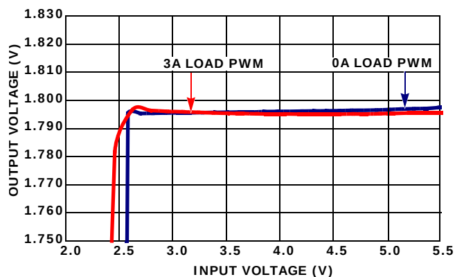
FIGURE 15. OUTPUT VOLTAGE REGULATION vs V_{\text{IN}} (PWM V_{\text{OUT}} = 1.8 )
