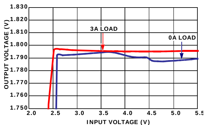
FIGURE 16. OUTPUT VOLTAGE REGULATION vs V_{\text{IN}} (PFM V_{\text{OUT}} = 1.8\text{V} )
