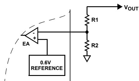
FIGURE 29. EXTERNAL RESISTOR DIVIDER
