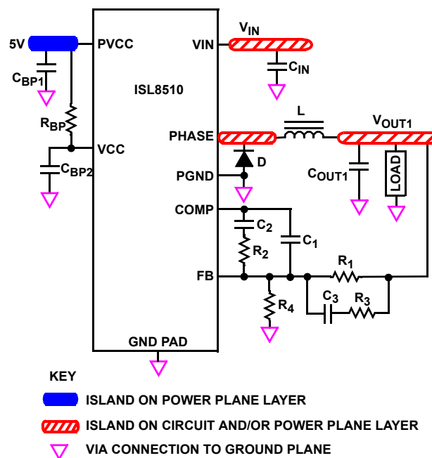
FIGURE 32. PRINTED CIRCUIT BOARD POWER PLANES AND ISLANDS
