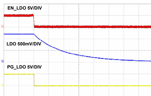
FIGURE 25. SHUT DOWN CIRCUIT, 20 \mu S/DIV
