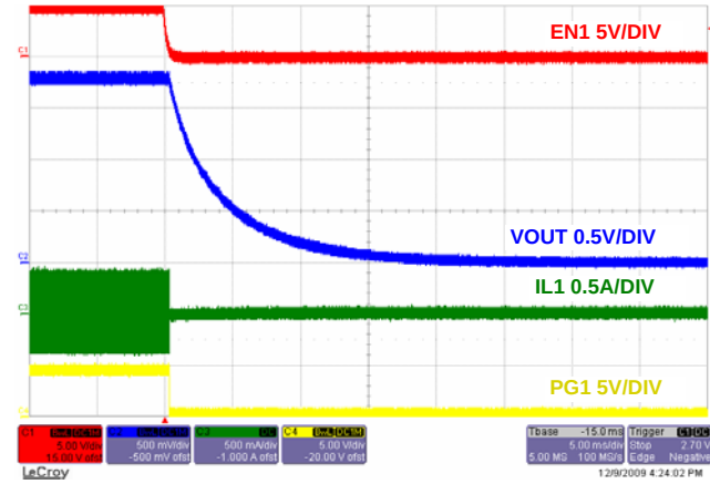
FIGURE 57. SOFT-DISCHARGE SHUTDOWN CHANNEL 1
