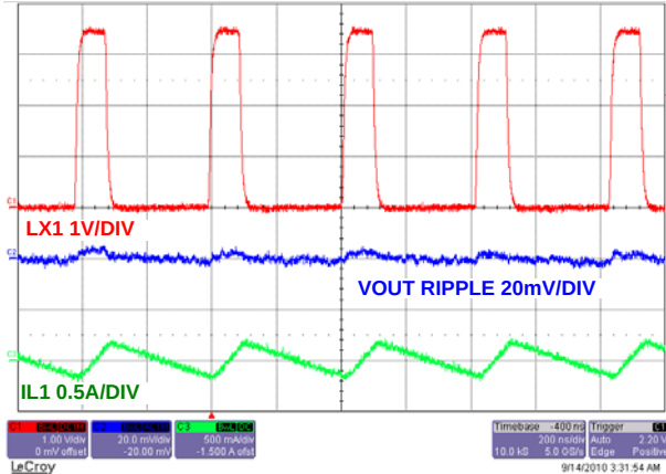
FIGURE 37. STEADY STATE OPERATION AT NO LOAD CHANNEL 2
