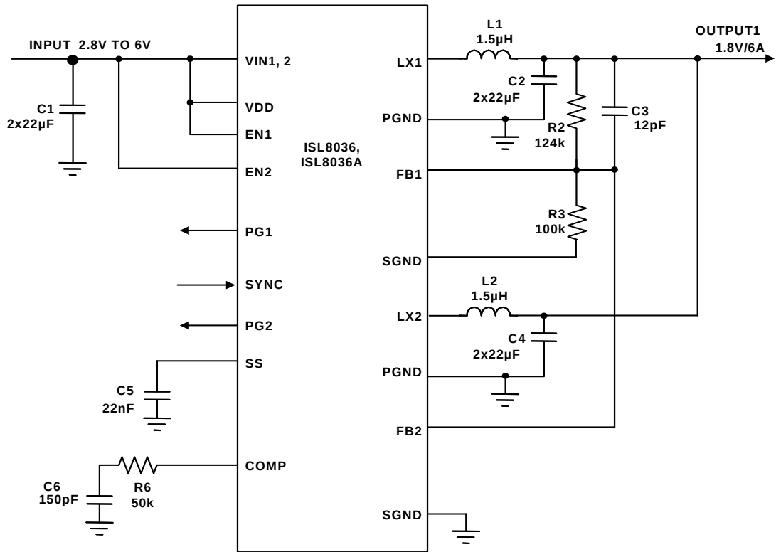
FIGURE 2. TYPICAL APPLICATION DIAGRAM - SINGLE 6A
