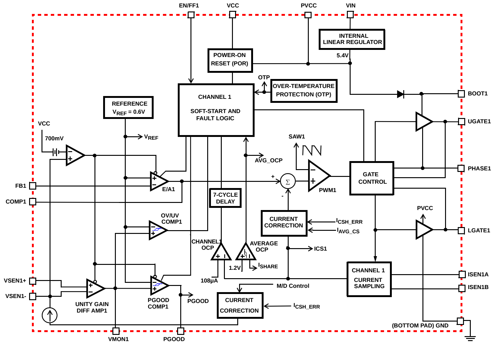
FIGURE 1. CHANNEL/PHASE 1 (VDDQ)
