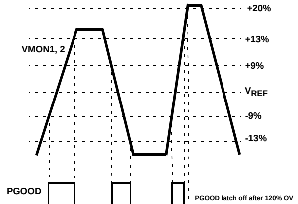
FIGURE 10. POWER-GOOD THRESHOLD WINDOW
