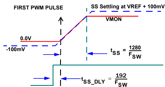
FIGURE 13. SOFT-START WITH V_{OUT} = 0V
