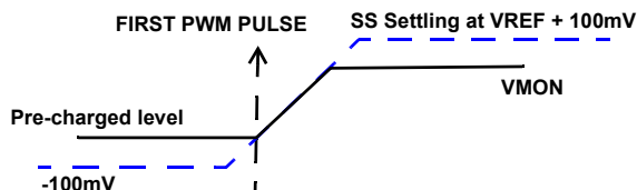
FIGURE 14. SOFT-START WITH OUTPUT PRE-CHARGED LEVEL < FINAL TARGET LEVEL
