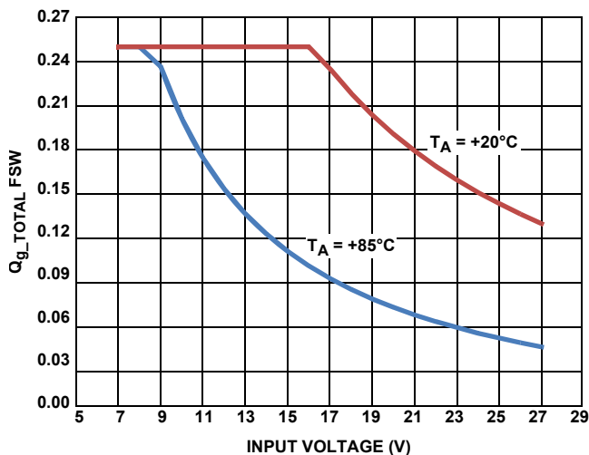
FIGURE 27. ALLOWED MAXIMUM GATE CHARGE vs INPUT VOLTAGE
