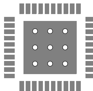
FIGURE 34. PCB VIA PATTERN
