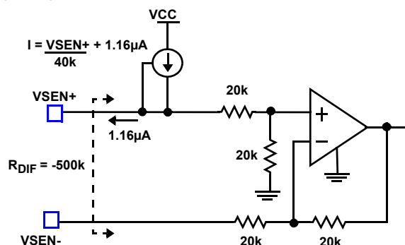
FIGURE 30. EQUIVALENT DIFFERENTIAL AMPLIFIER
