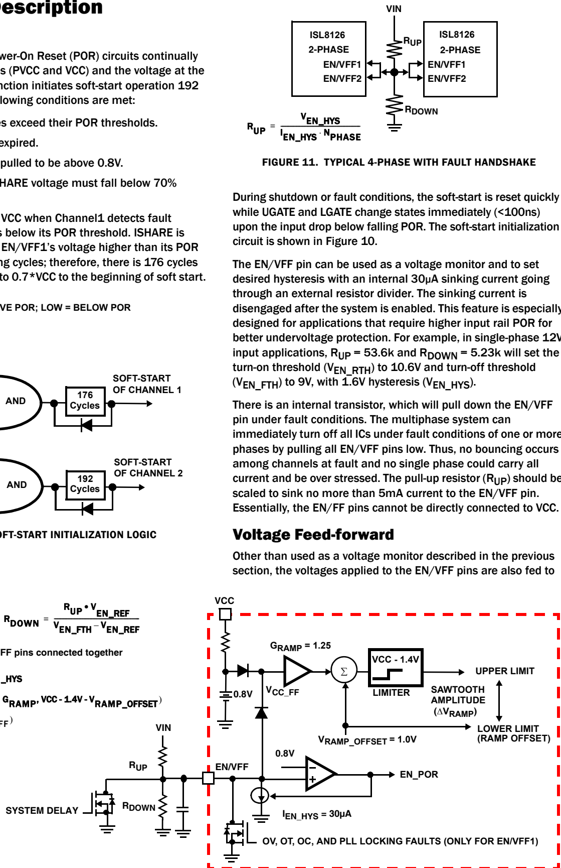
FIGURE 12. SIMPLIFIED ENABLE AND VOLTAGE FEEDFORWARD CIRCUIT
