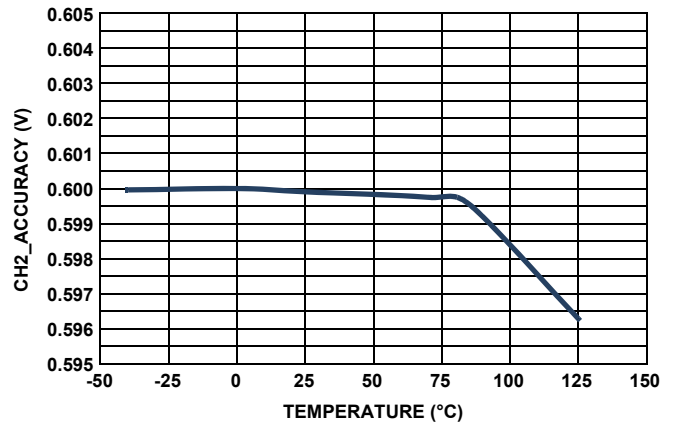
FIGURE 2. CHANNEL 2 ACCURACY vs TEMPERATURE
