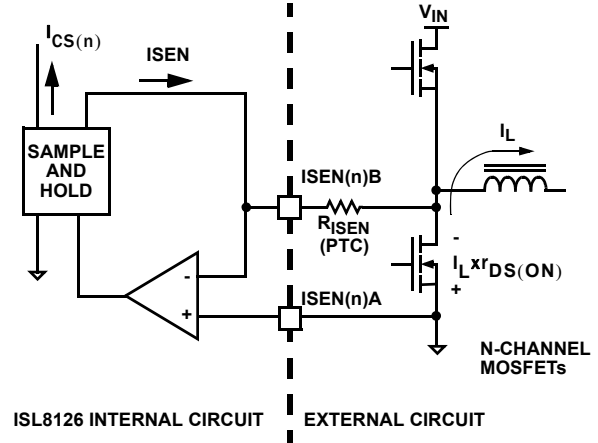
FIGURE 21. MOSFET r_{DS(ON)} CURRENT-SENSING CIRCUIT
