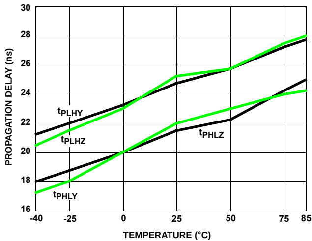
FIGURE 12. DRIVER PROPAGATION DELAY vs TEMPERATURE (ISL81487E)
