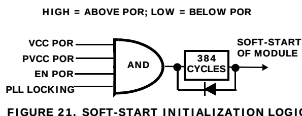
FIGURE 21. SOFT-START INITIALIZATION LOGIC
