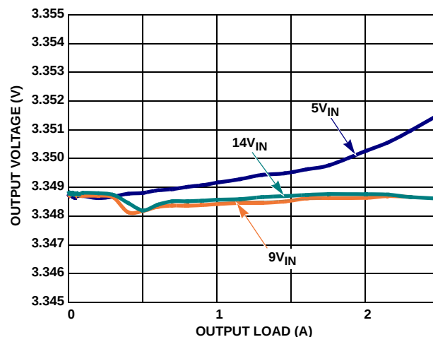
FIGURE 12. V_{OUT} REGULATION vs LOAD ( V_{OUT} = 3.3V , 500kHz)
