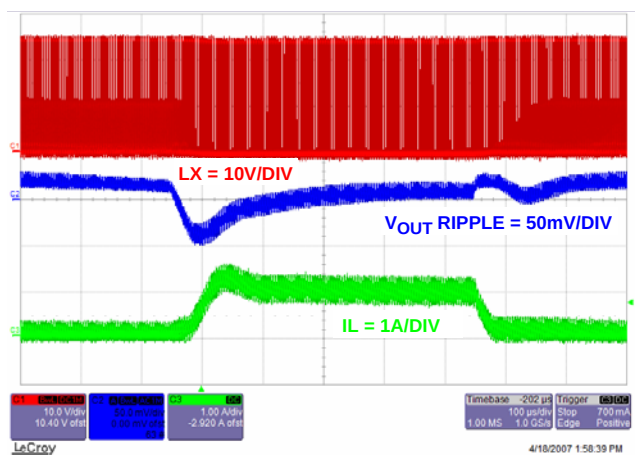
FIGURE 21. LOAD TRANSIENT
