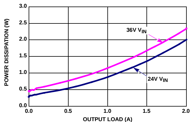
FIGURE 17. POWER DISSIPATION vs LOAD ( V_{OUT} = 12V - 500kHz )
