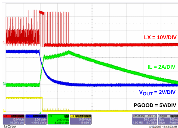
FIGURE 25. OUTPUT SHORT CIRCUIT
