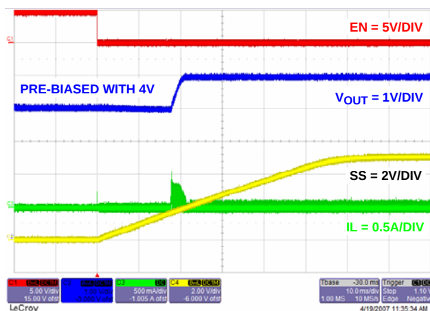
FIGURE 23. SOFT-START WITH PRE-BIASED
