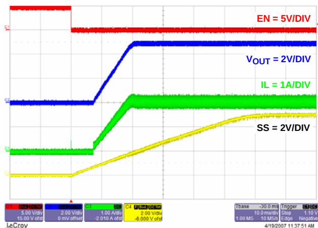
FIGURE 24. SOFT-START AT FULL LOAD
