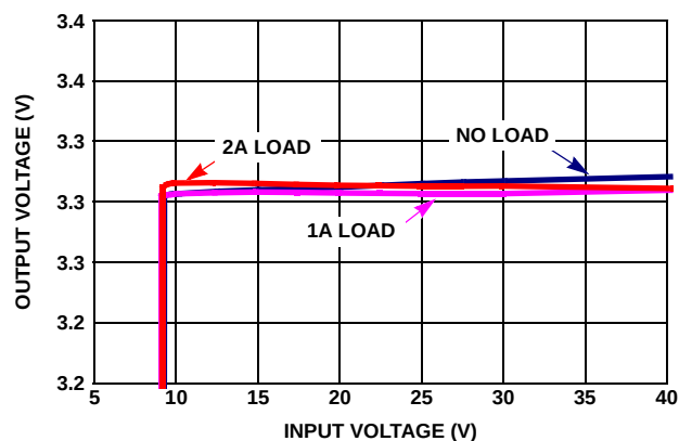
FIGURE 11. OUTPUT VOLTAGE REGULATION vs V_{IN} PWM MODE
