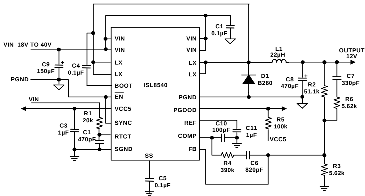
FIGURE 3. TYPICAL SCHEMATIC FOR ISL8540 (12V V_{OUT} )
