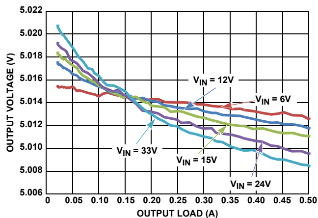
FIGURE 26. V_{OUT} REGULATION vs LOAD, PWM, V_{OUT} = 5\text{V}
