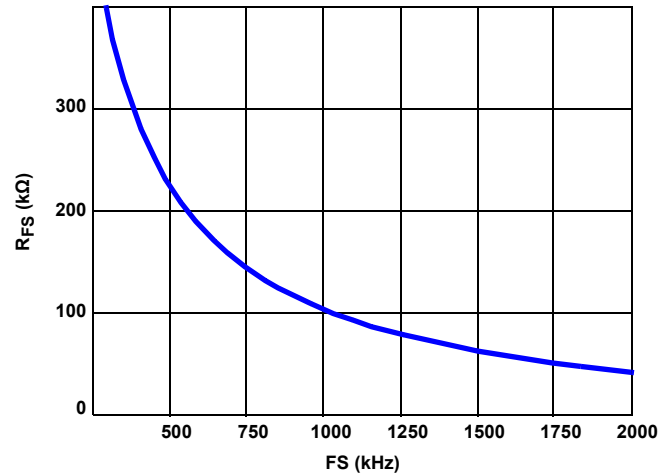
FIGURE 59. R_{FS} SELECTION vs F_S
