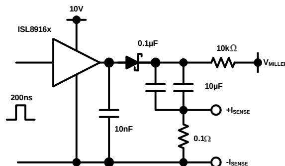
FIGURE 6. MILLER PLATEAU SOURCE CURRENT TEST CIRCUIT
