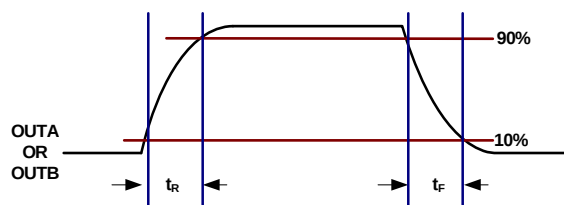
FIGURE 4. RISE/FALL TIMES
