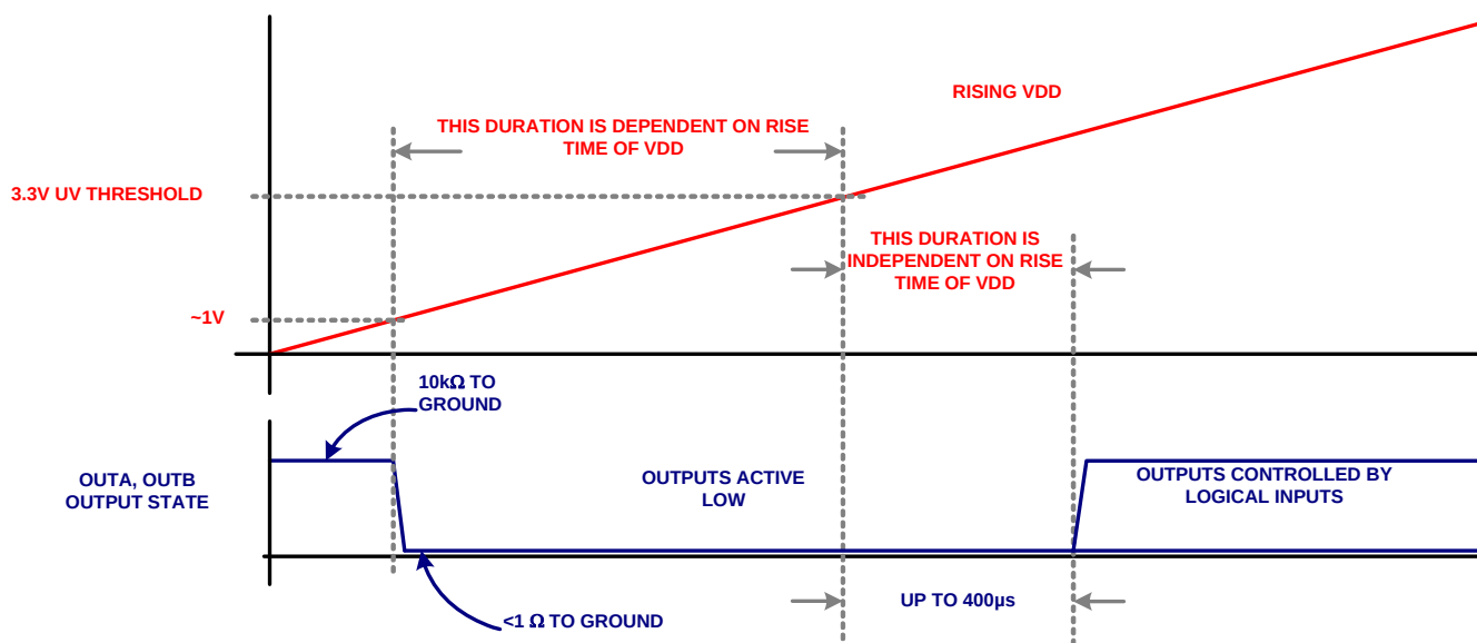
FIGURE 9. START-UP SEQUENCE
