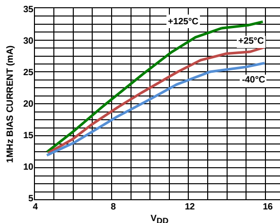
FIGURE 11. I_{DD} vs V_{DD} (1MHz)
