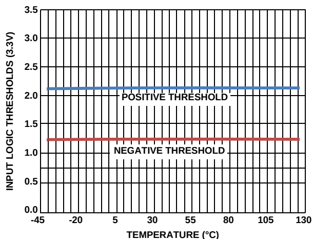
FIGURE 14. INPUT THRESHOLDS
