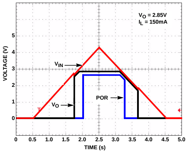
FIGURE 12. POWER-UP/POWER-DOWN
