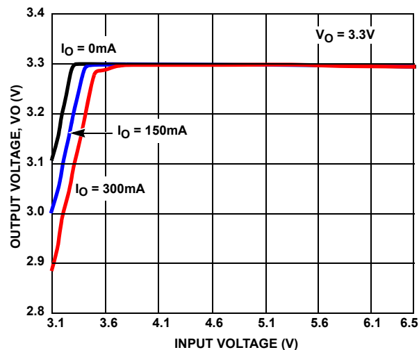
FIGURE 5. OUTPUT VOLTAGE vs INPUT VOLTAGE (3.3V OUTPUT)
