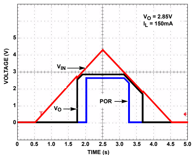
FIGURE 12. POWER-UP/POWER-DOWN
