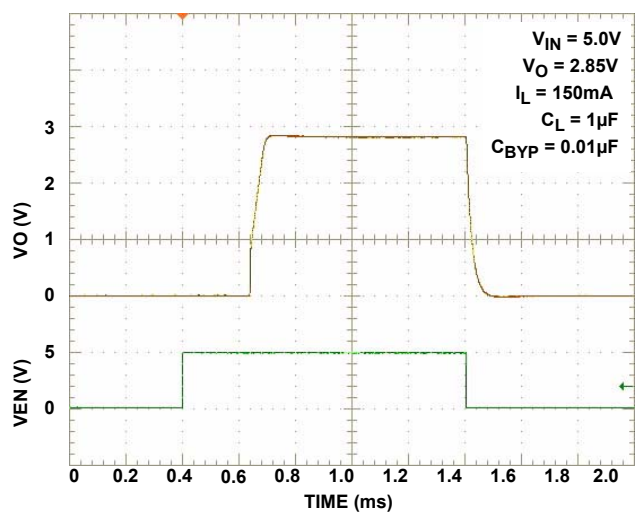
FIGURE 13. TURN-ON/TURN-OFF RESPONSE
